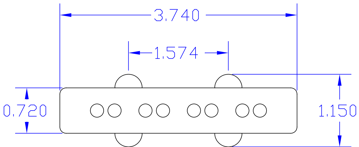
AGUILAR AG 4J BRIDGE PICKUP COVER
